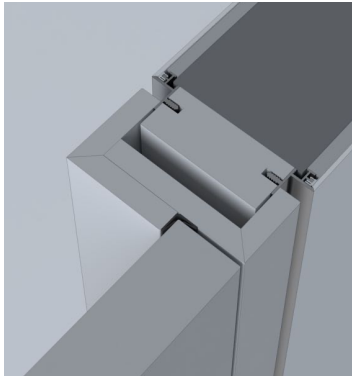
Section of a L shape door jamb with one side adjustable casing, installed on shadow gap subframe.
