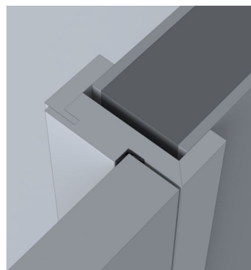
Section of a L shape door jamb with one side adjustable casing, installed on normal masonry or dry wall.
