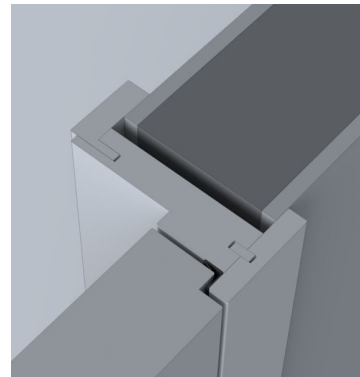
Section of a full casing-covered jamb on one side and an adjustable jamb on the other side, outside flush swing-in.
